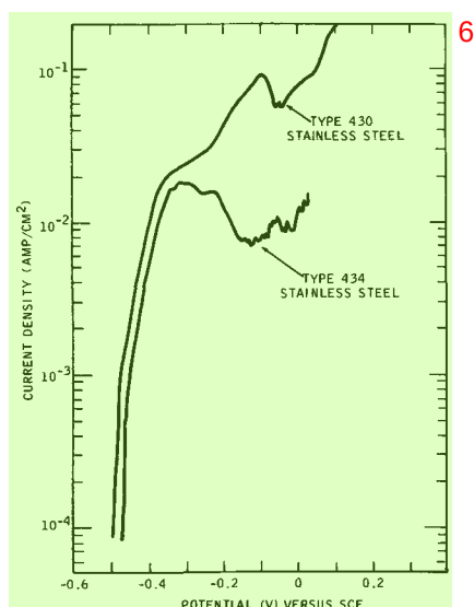
Fig. 5. Anodic potentiodynamic polarization curves for Types 430 and 434 stainless steels in 1N hydrochloric acid at 29.6°C (unmasked electrodes).
