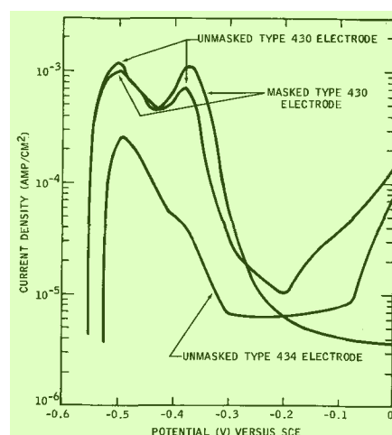
Fig. 1. Anodic potentiodynamic polarization curves for unmasked Types 430 and 434 electrodes and for masked Type 430 electrode in 0.1N hydrochloric acid at 29.6°C. 14
