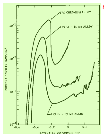
Fig. 6. Anodic potentiodynamic polarization curves for 17% chromium, 17% Cr-1% Mo, and 17% Cr-3% Mo alloys in 1N hydrochloric acid at 29.6°C (unmasked electrodes).
