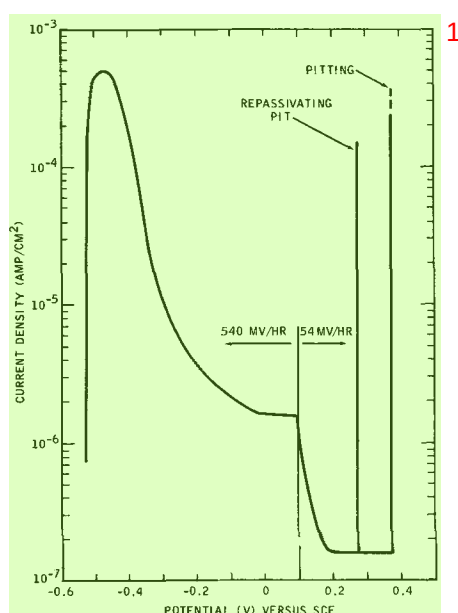
Fig. 4. Anodic potentiodynamic polarization curve for masked 17% Cr-1% Mo electrode in 0.1N hydrochloric acid at 29.6°C.
